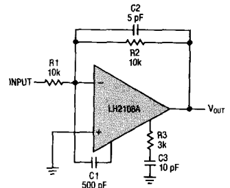
Feedforward Compensation
