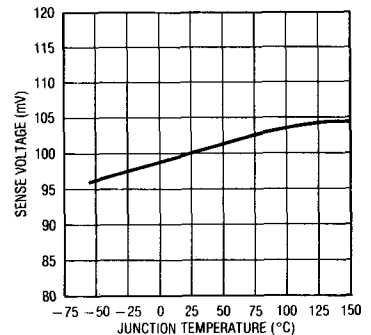
Current Limit Comparator Sense Voltage
