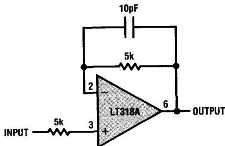
Voltage Follower
