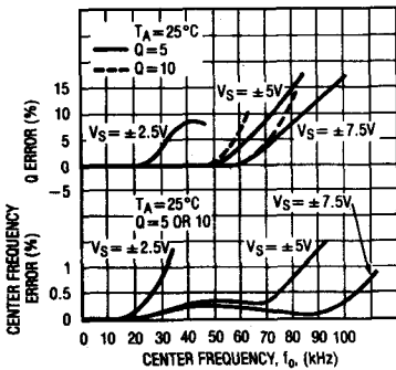
Graph 1. Mode 1, (f_{CLK}/f_0) = 50:1
