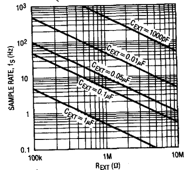
Sampling Rate vs R EXT , C EXT
