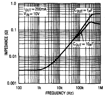
Output Impedance
