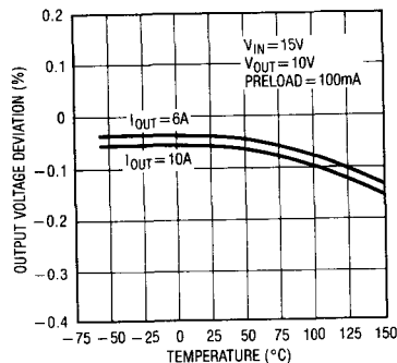
Load Regulation
