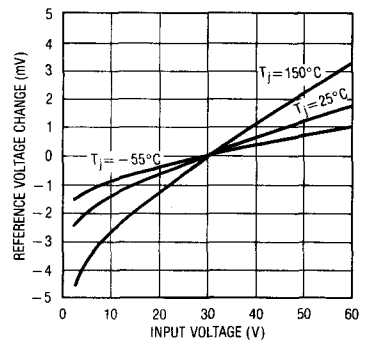
Line Regulation
