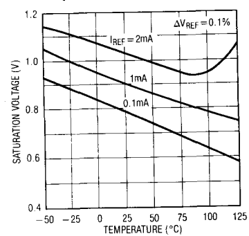
Output Saturation
