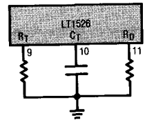
Oscillator Connections
