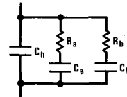
Typical Hold Capacitor Equivalent Circuit
