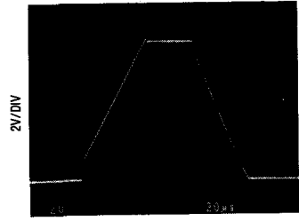
A_V = +1 , 20\mu\text{s}/\text{DIV}
