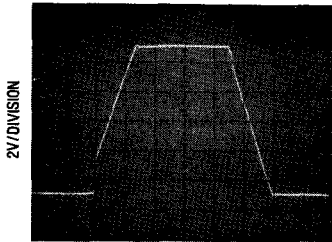
A_V = +1, C_S = 100\text{pF}, 20\mu\text{sec/DIV}
