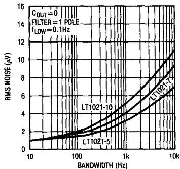
Output Voltage Noise
