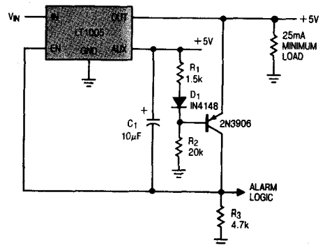
Latch-Off for V_{OUT} \leq 4.7V
