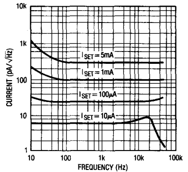
Current Noise
