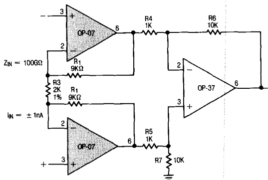
Instrumentation Amplifier
