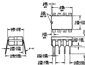
J8 Package 8 Lead Hermetic Dip
