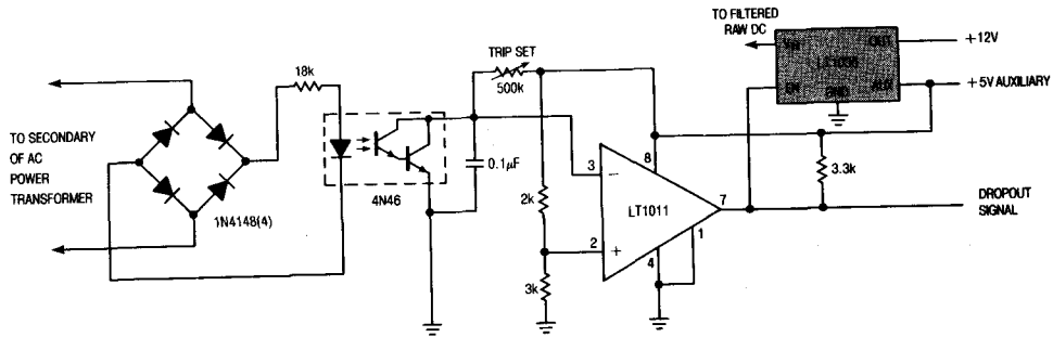
Line Dropout Detector
