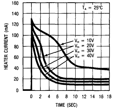
Heater Current
