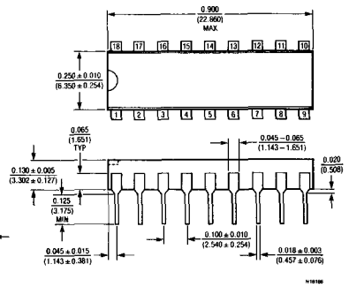
N Package 18-Lead Plastic DIP
