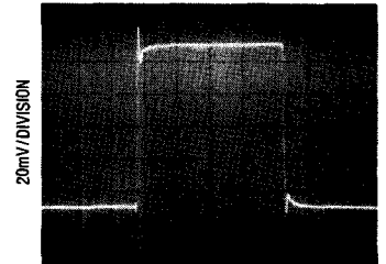
A_V = +1, C_I = 30\text{pF}, C_{LOAD} = 100\text{pF}, 5\mu\text{sec/DIV}
