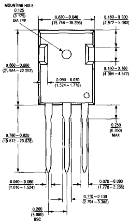
P Package TO-3P Plastic
