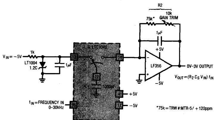
0.005% F → V Converter
