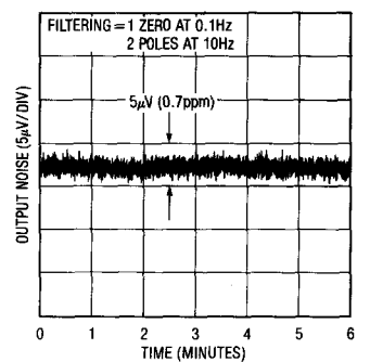
Output Noise 0.1Hz to 10Hz LT1021-7
