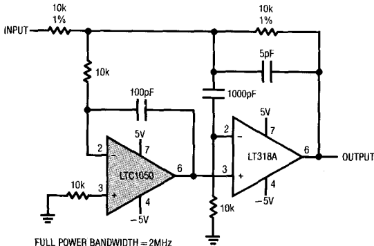
Fast Precision Inverter
