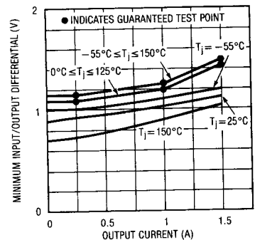
LT1086 Dropout Voltage
