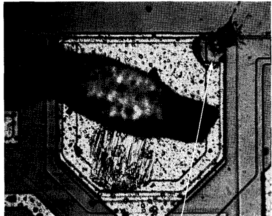
RESISTIVE SHORT ON A METALLIZATION STRIP OVER A THIN OXIDE \text{N}^+ REGION ON A BIPOLAR IC
