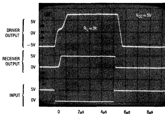
Output Waveform
