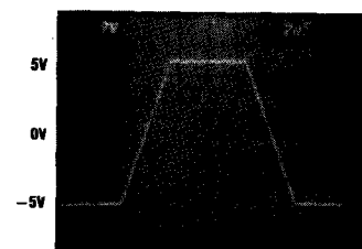
LT1007 Large Signal Response
