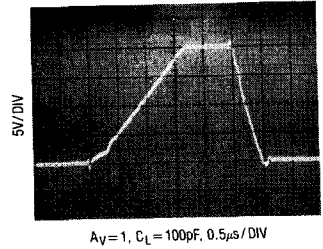
LT1055 Large Signal Response
