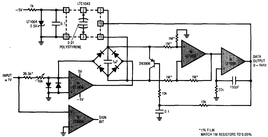
12 Bit A-D Converter
