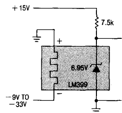
Portable Calibrator
