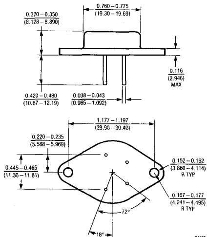
TO-3 Type Metal Can (Steel) K Package
