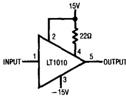
LT1010 Buffer†
