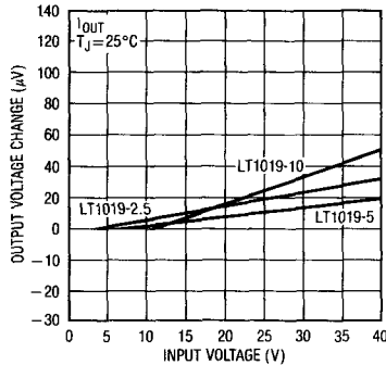
Line Regulation
