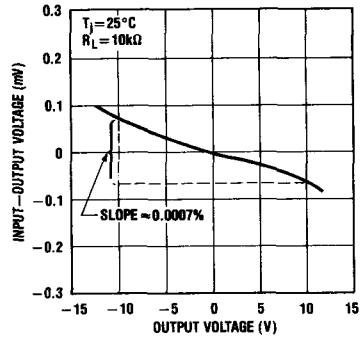
Gain Error
