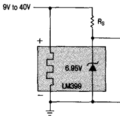
Single Supply Operation
