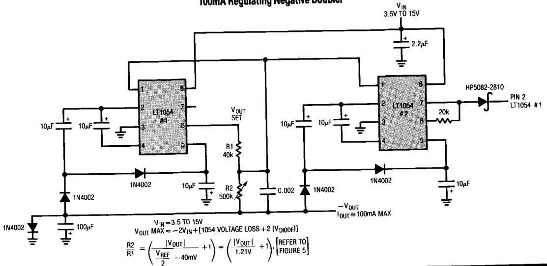
100mA Regulating Negative Doubler
