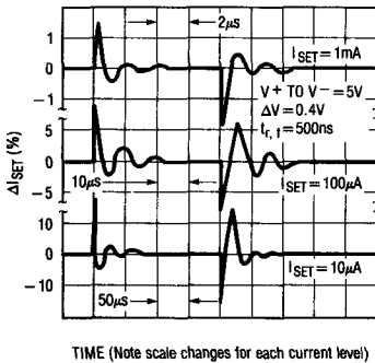
Transient Response
