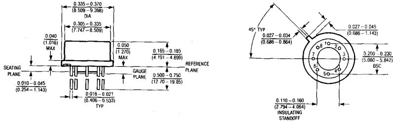
H Package TO-5 Metal Can
