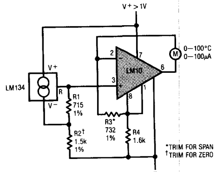
Thermometer
