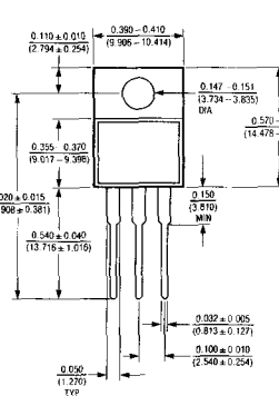
T Package TO-220 Plastic
