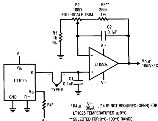
Type K 10mV/°C Thermometer
