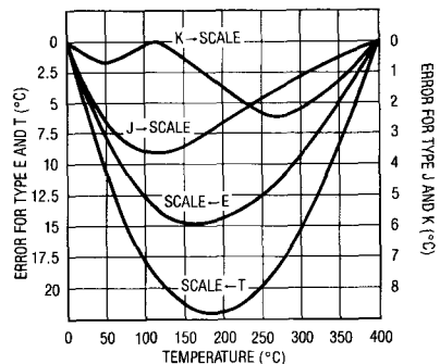
Figure 4. Thermocouple Nonlinearity, 0°C–400°C
