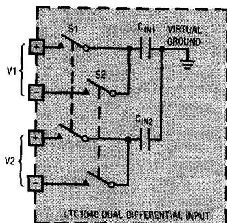
Figure 2. Dual Differential Equivalent Input Circuit
