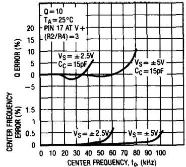
Graph 3. Mode 2, (f_{CLK}/f_0) = 25:1
