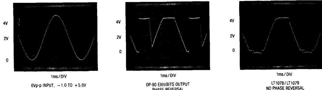
Voltage Follower with Input Exceeding the Negative Common-Mode Range ( V_S = 5V, 0V )
