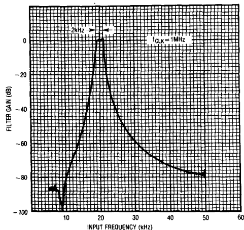
Amplitude Response
