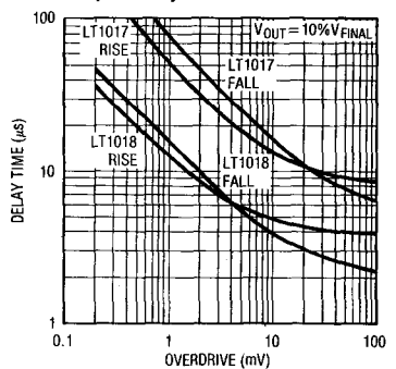
Output Delay
