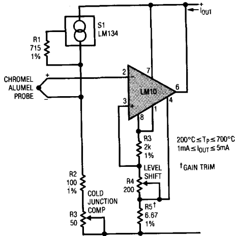
Thermocouple Transmitter
