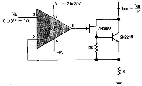
Precision Current Sink
