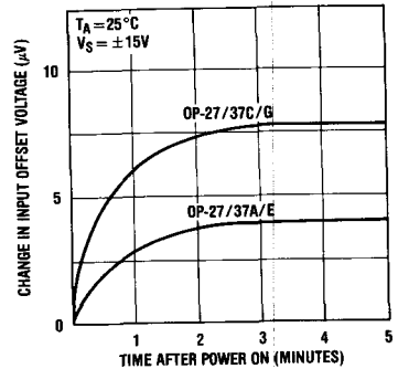
Warm-Up Drift
