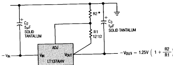
Negative Regulator
