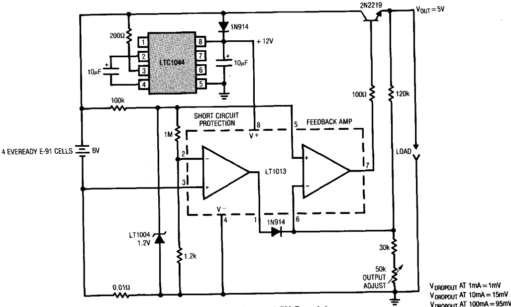
Figure 17. Low Dropout 5V Regulator
