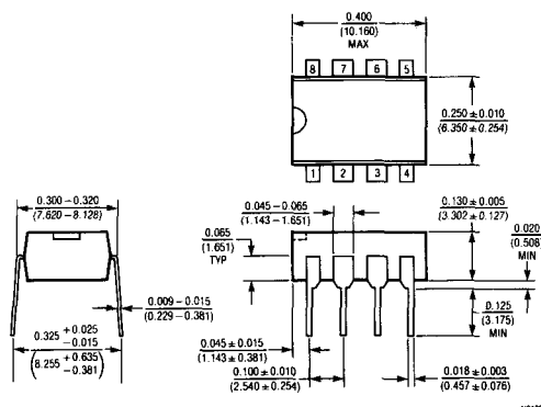
N Package 8-Lead Plastic MiniDIP
