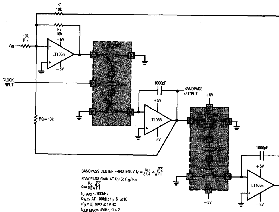
High Frequency Clock Tunable Bandpass Filter
