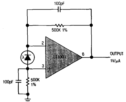
Photodiode Amplifier
