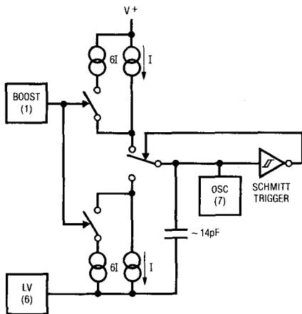
Figure 5. Oscillator
