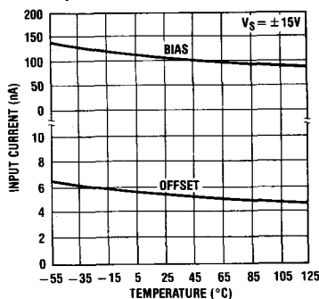
Input Current
