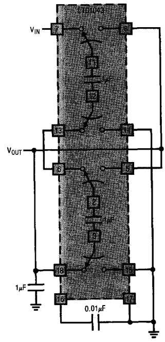
Divide by 4
