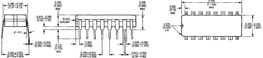
J Package 16-Lead Ceramic DIP
