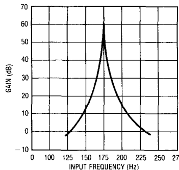
Amplitude Response
