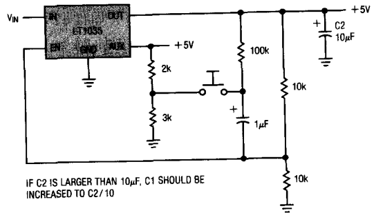
Push-On, Push-Off
