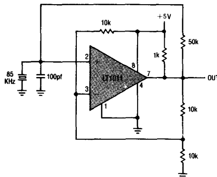
Crystal Oscillator
