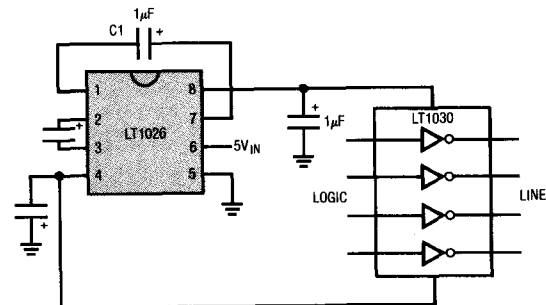
5V Powered RS232 Line Driver
