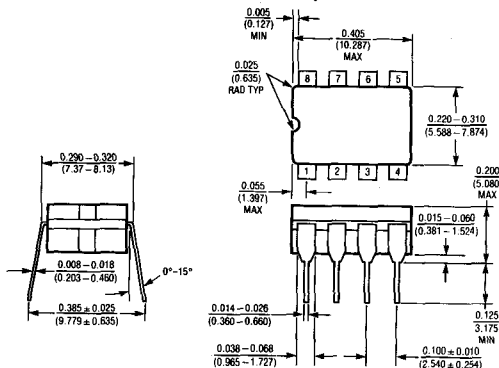
J Package 8 Lead Cerdip
