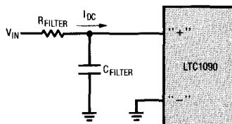
Figure 13. RC Input Filtering
