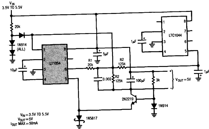
Regulating 200mA +12V to -5V Converter
