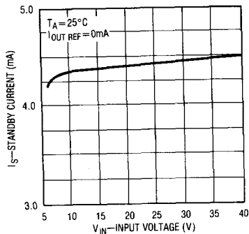
Standby Current
