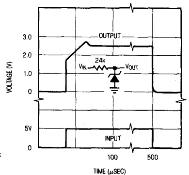
Response Time
