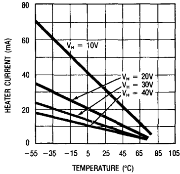
Heater Current
