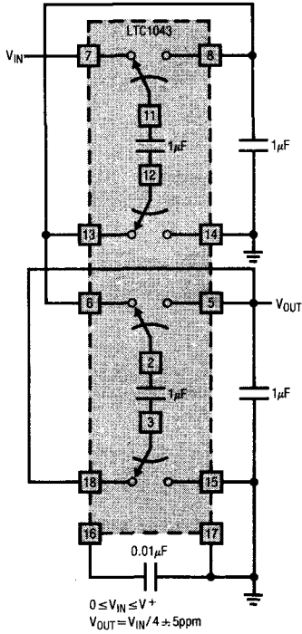
Divide by 4
