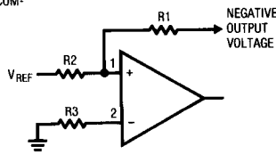
Error Amplifier Connections
