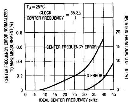
Center Frequency and Q Error
