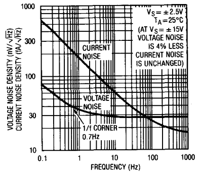
Noise Spectrum
