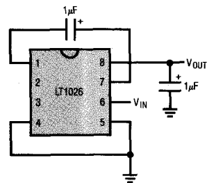
Voltage Doubler
