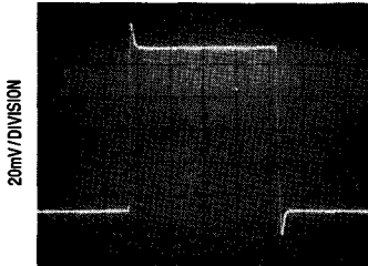
A_V = +1, C_S = 100\text{pF}, C_{LOAD} = 100\text{pF}, 5\mu\text{sec/DIV}
