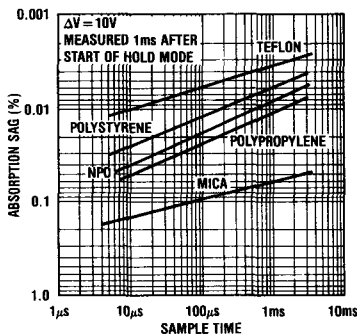
Capacitor Dielectric Absorption
