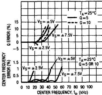
Graph 2. Mode 1, (f_{CLK}/f_0) = 100:1
