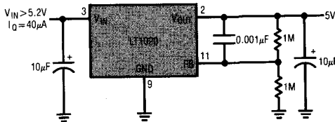
5V Regulator
