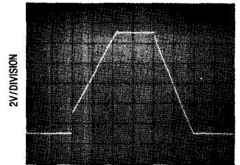
A_V = +1, C_I = 30\text{pF}, 20\mu\text{sec/DIV}
