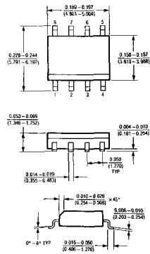
SO Package 8-Lead Plastic SOIC
