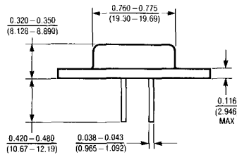
K Package 4 Lead TO-3 Metal Can
