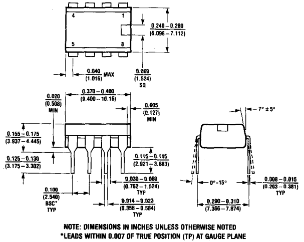
N8 Package 8 Lead Plastic
