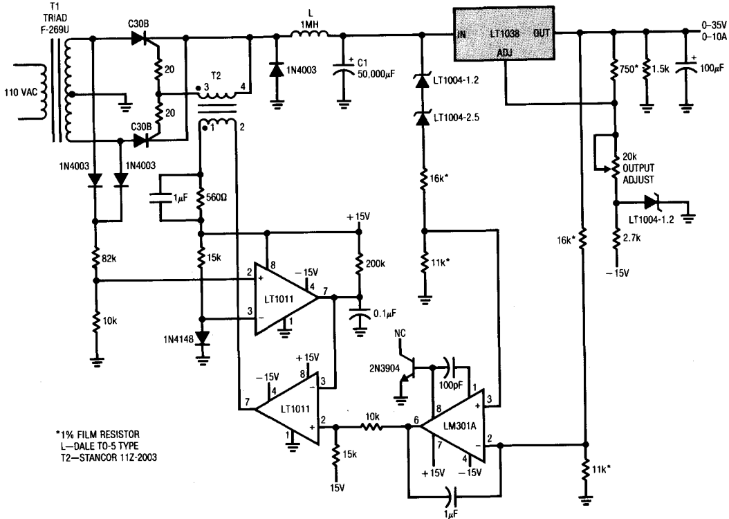
10 Amp Variable Regulator*
