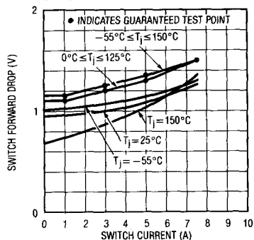
LT1089 Switch Voltage vs Output Current
