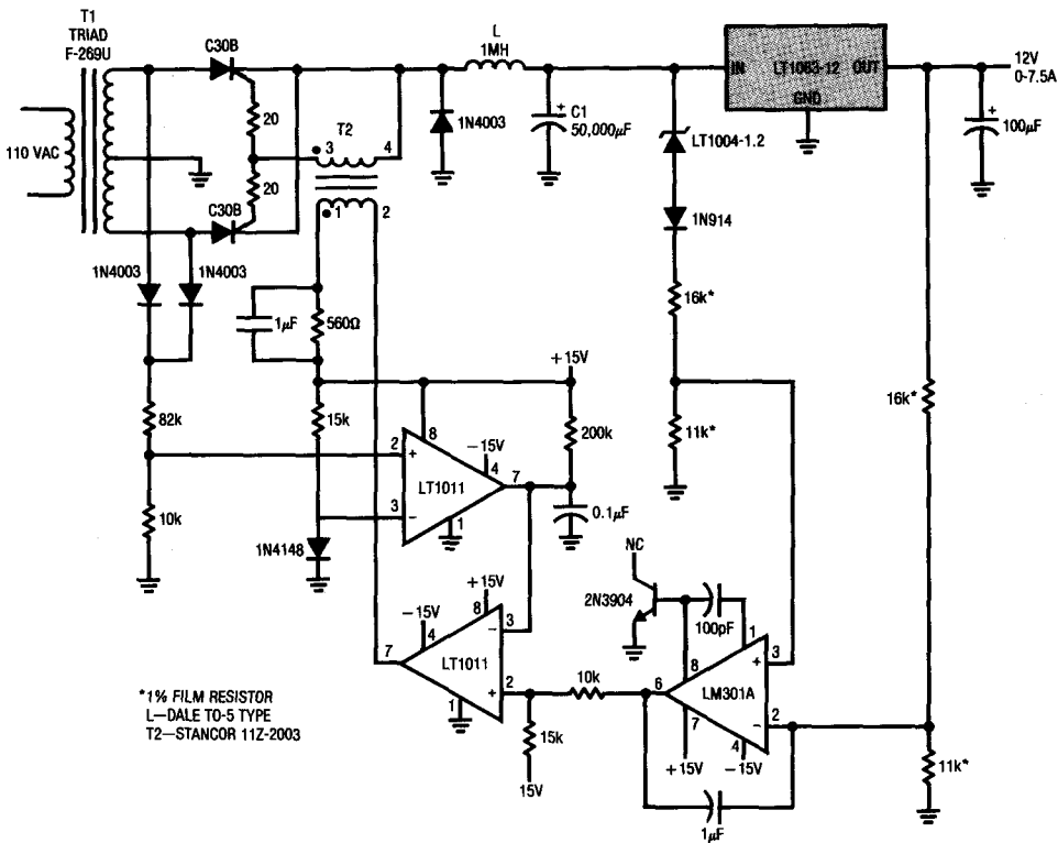
REGULATOR WITH SCR PREREGULATOR TO LOWER POWER DISSIPATION. ABOUT 1.7V DIFFERENTIAL IS MAINTAINED ACROSS THE LT1083 INDEPENDENT OF LOAD CURRENT.
