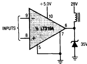
Relay Driver
