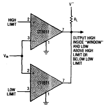
Window Detector
