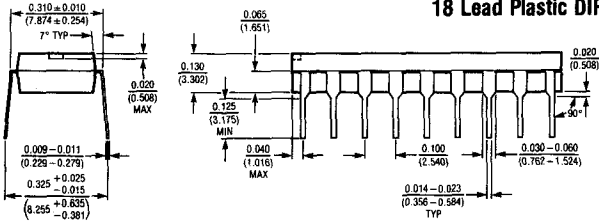
N Package 18 Lead Plastic DIP
