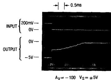
Overload Recovery
