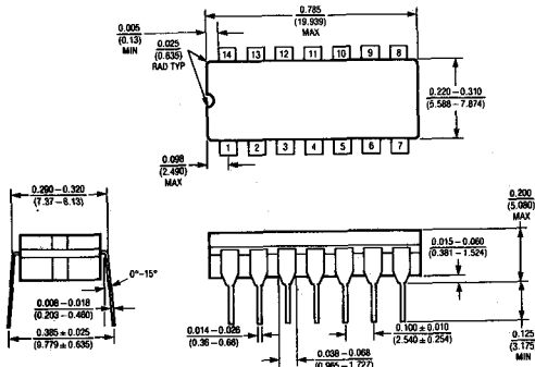
J Package 14-Lead Ceramic DIP
