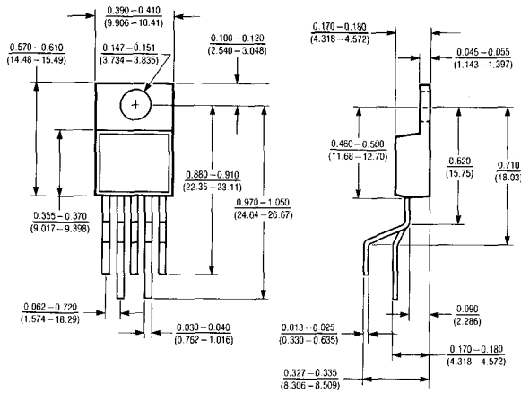
TO-220 Package (5 Lead)
