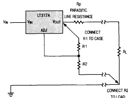
Connections for Best Load Regulation
