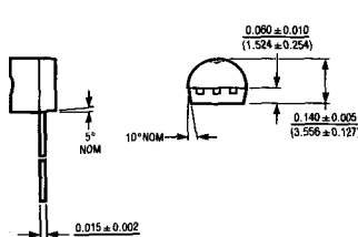
Z Package Plastic
