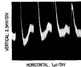
Figure 16. Poor Reference Settling Can Cause A/D Errors
