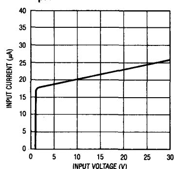
Input Current
