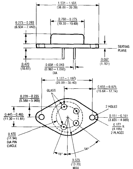
4-Pin Metal Package Similar to JEDEC TO-3
