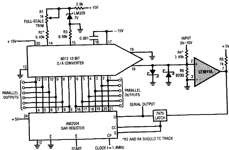
10 \mu s 12-Bit A-D Converter
