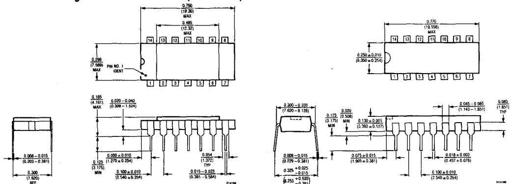
D14 Package 14-Lead Hermetic DIP (Sidebrazed)
