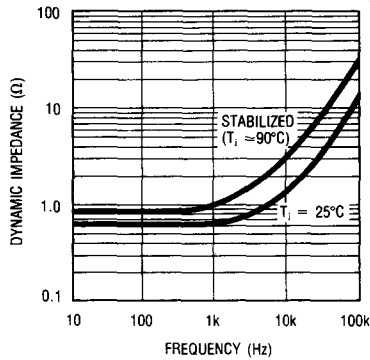
Dynamic Impedance
