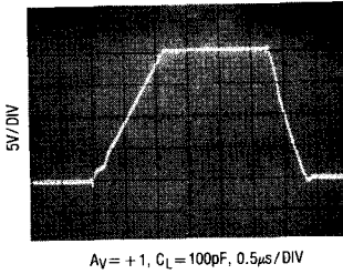
LT1056 Large Signal Response
