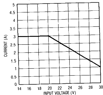
Guaranteed Load Current, 12V Output
