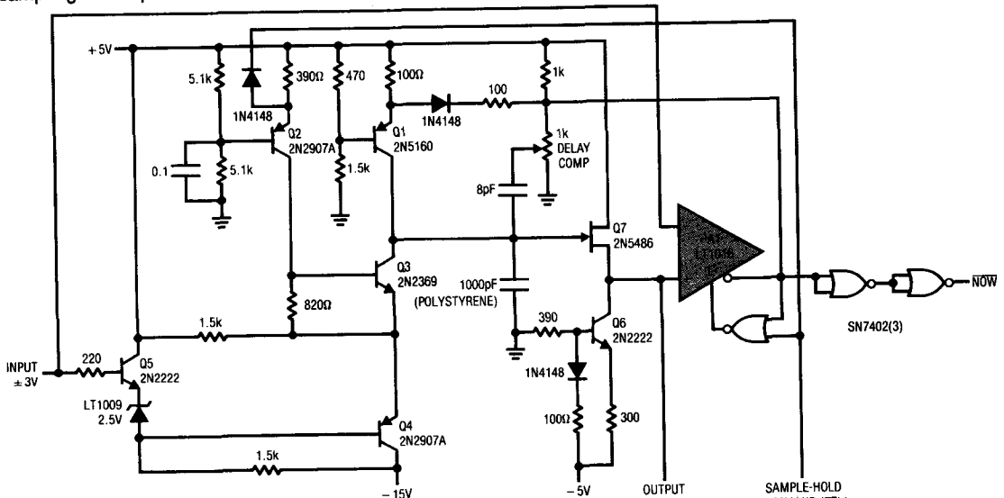
Figure 14. 200ns Sample-and Hold
