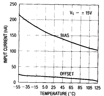
Input Currents
