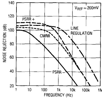
Noise Rejection
