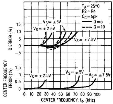
Graph 6. Mode 3, ( f_{CLK}/f_o ) = 50:1
