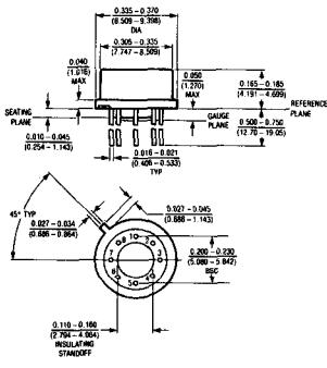
H Package Metal Can
