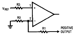
Error Amplifier Connections
