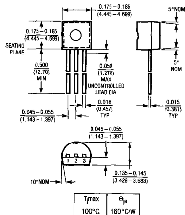
Z Package, 3 Lead TO-92 Plastic
