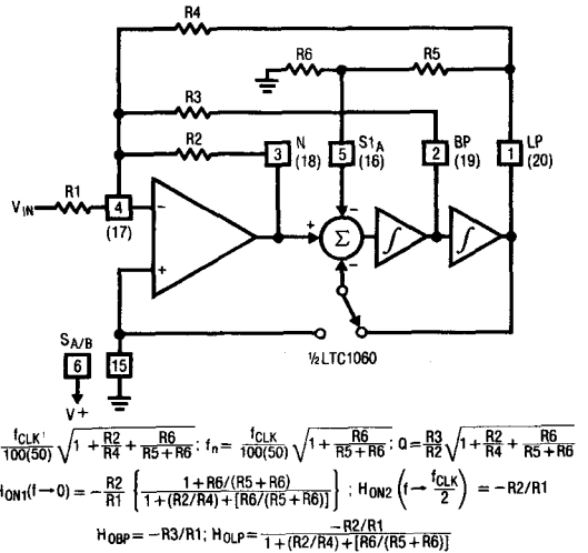
Figure 9. Mode 2a: 2nd Order Filter Providing Notch, Bandpass, Lowpass
